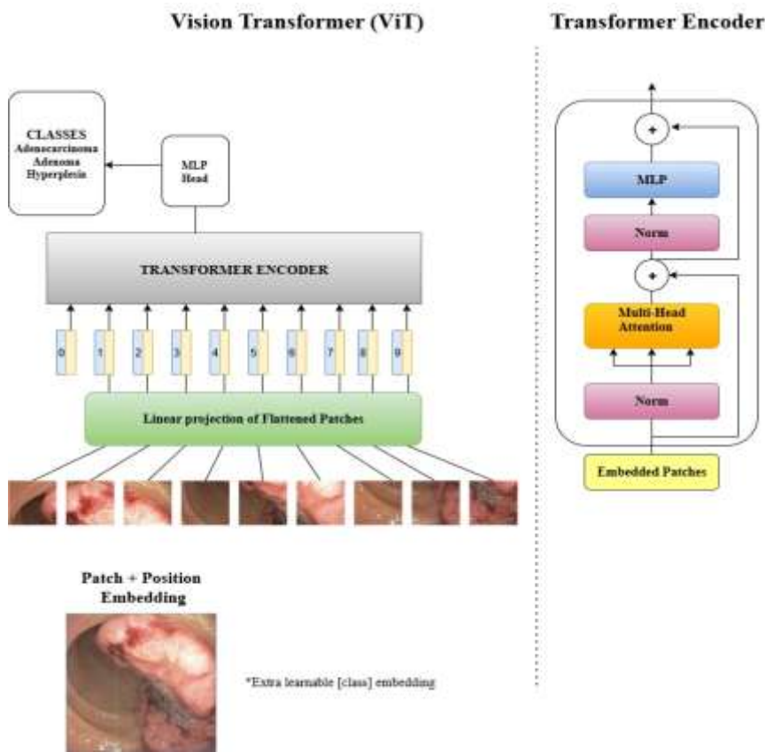
Figure 2. ViT Architecture.
