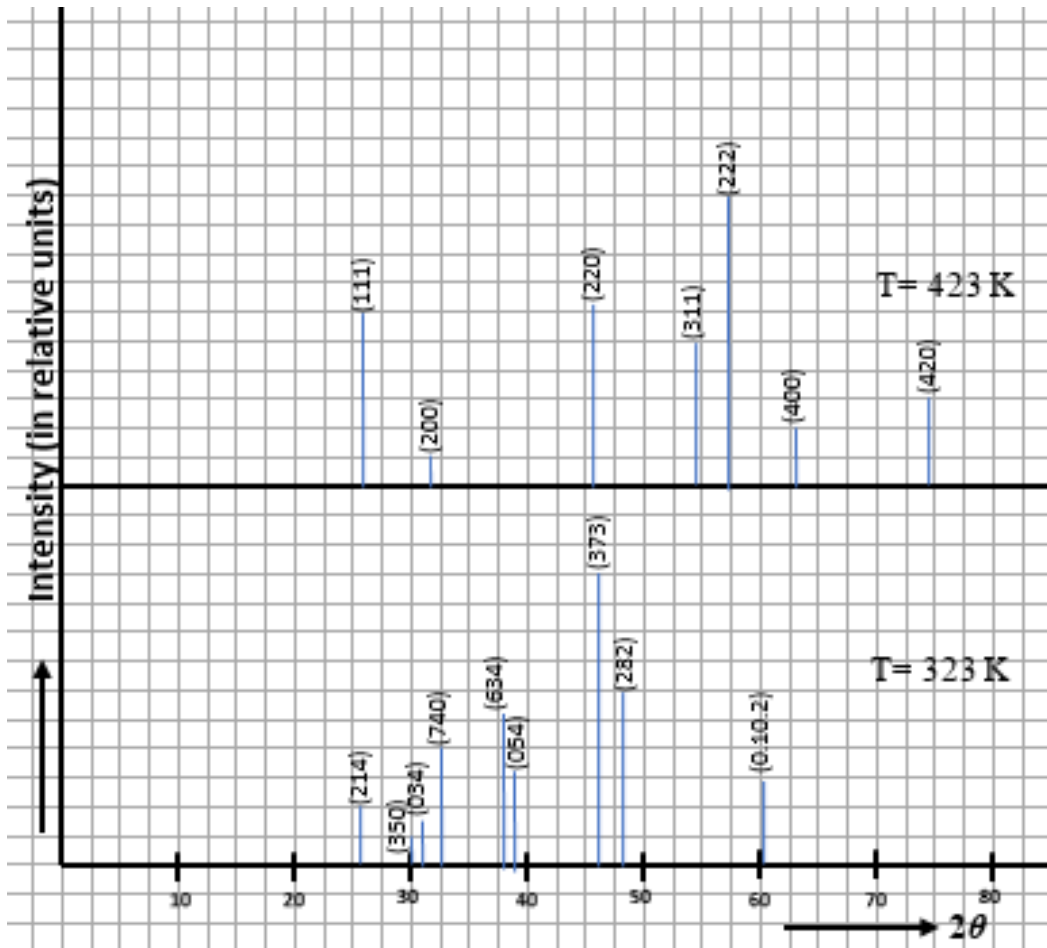
Figure 1. Diffractogram of Cu 1.70 Ni 0.05 S crystal
