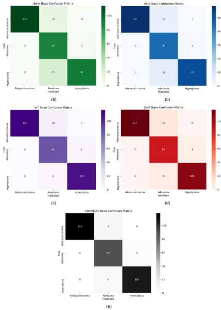
Figure 3. Confusion matrices of ViT Models: (a) Swin Base, (b) , BeiT Base (c) ViT Base, (d) DeiT Base, (e) ConvNeXt Base.
